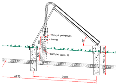
Fig. 7 - Principle for vertical introduction to the solar panel
